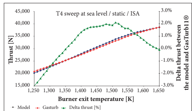
Figure 10. Three shaft simulated engine thrust comparison.
